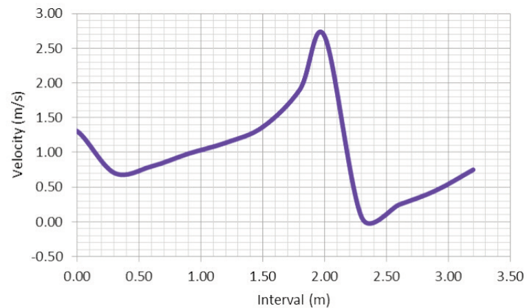
Figure 8: Graphic presentation of vertical air velocity in the flue at different height intervals for a summer day.
