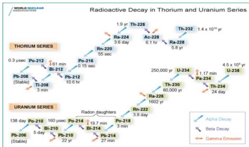
Figure 1—Radioactive decay in the Th and U series
