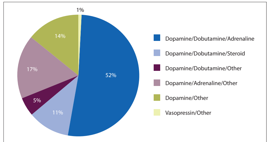
Fig. 1. Antihypotensive combinations.
