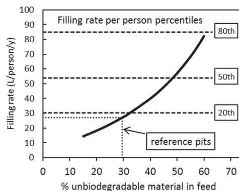
Figure 13 Average filling rates per person vs. feed composition, including coarse refuse
