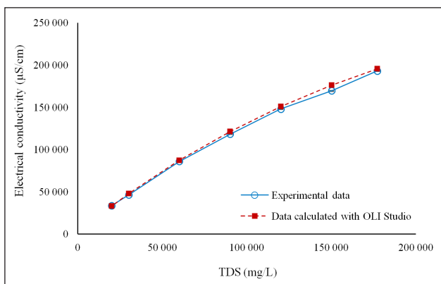
Figure 3. Curves of electrical conductivity as a function of total dissolved solids experimentally obtained and calculated with OLI Studio for Field D brine (TDS range: from 20 000 to 177 085 mg/L). The error bars on the experimental data indicate the standard error of the mean for the triplicate experiments
