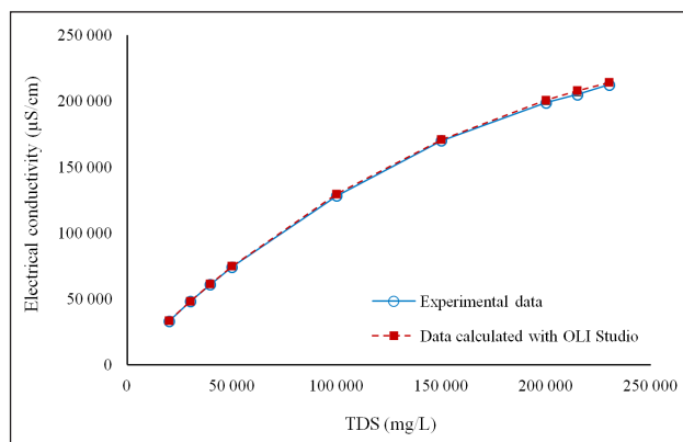
Figure 4. Curves of electrical conductivity as a function of total dissolved solids experimentally obtained and calculated with OLI Studio for concentrated DSW (TDS range: from 20 000 to 230 000 mg/L). The error bars on the experimental data indicate the standard error of the mean for the triplicate experiments
