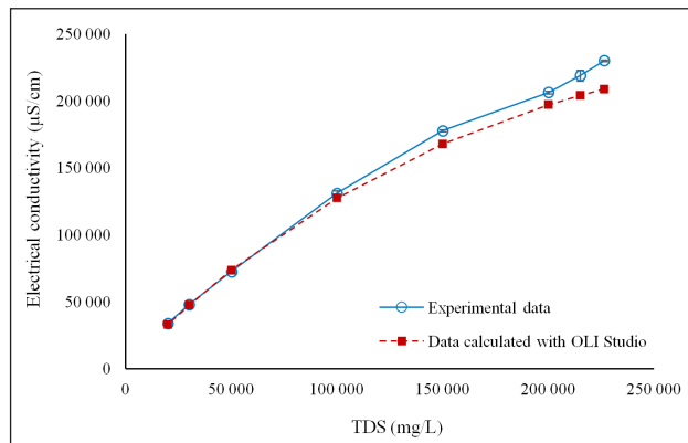
Figure 2. Curves of electrical conductivity as a function of total dissolved solids experimentally obtained and calculated with OLI Studio for Field B brine (TDS range: from 20 000 to 226 365 mg/L). The error bars on the experimental data indicate the standard error of the mean for the triplicate experiments
