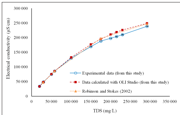
Figure 1. Curves of electrical conductivity as a function of total dissolved solids experimentally obtained and calculated with OLI Studio (both from this study) and that provided by Robinson and Stokes (2002) for aqueous sodium chloride solutions. The error bars on the experimental data indicate the standard error of the mean for the triplicate experiments
