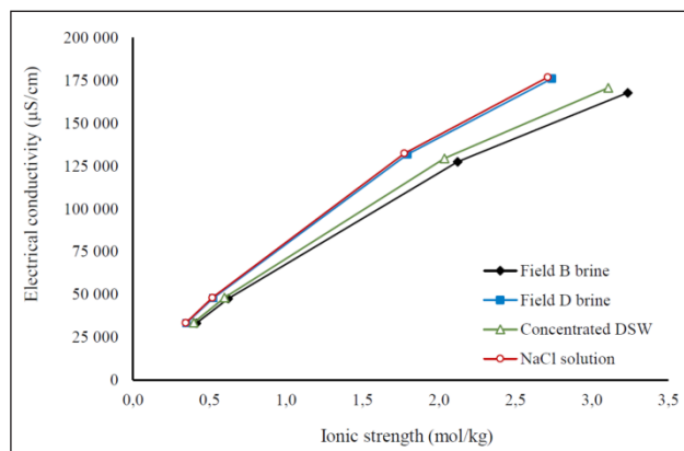
Figure 6. Curves of electrical conductivity as a function of ionic strength for all aqueous solutions using data calculated with OLI Studio
