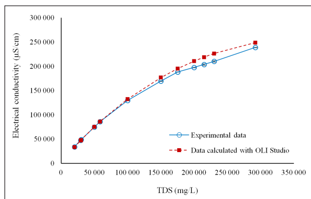
Figure 5. Curves of electrical conductivity as a function of total dissolved solids experimentally obtained and calculated with OLI Studio for sodium chloride solution (TDS range: from 20 000 to 292 200 mg/L). The error bars on the experimental data indicate the standard error of the mean for the triplicate experiments
